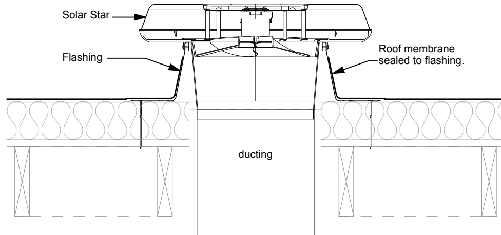
SECTION INSULATION OVER JOISTS
